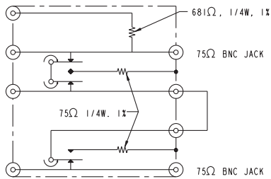
CIRCUIT SCHEMATIC
