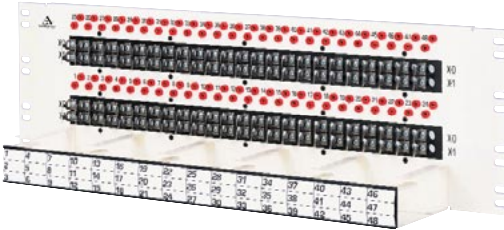
Module face plate available with and without lateral tabs, depending on spacing and number of modules per panel.
